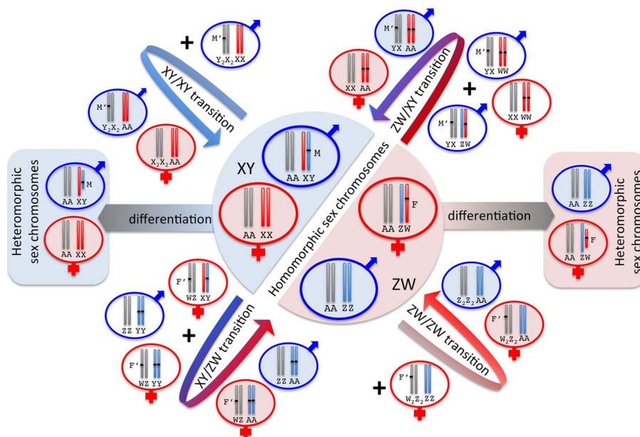
Figure 5. Transitions versus differentiation of sex chromosomes. Transitions between homomorphic sex chromosomes result from new masculinizing (M') or feminizing (F') mutations that invade an existing XY or ZW system to create a new chromosome pair (in grey) that harbors the sex-determining gene (additional transitional karyotypes are indicated by unshaded circles). XY→XY transitions result in the loss of the ancestral Y (and ZW→ZW transitions cause loss of the ancestral W). Transitions between XY and ZW systems result in some offspring that are homozygous for the Y (blue) or W (red) chromosome and are thus more likely if the chromosomes have similar gene content but become increasingly difficult if these chromosomes have degenerated (side boxes on left and right), causing YY and WW individuals to be less fit. doi:10.1371/journal.pbio.1001899.g005
