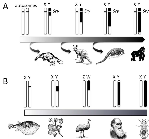
Figure 1. Sex chromosome differentiation. A. Reconstructed evolutionary path of sex chromosome differentiation in humans. Sex chromosomes originate from autosomes that acquired a sex-determining function (the Sry gene) after their split from monotremes. Suppression of recombination between the sex chromosomes, associated with degeneration of the non-recombining region of the Y chromosome, results in the morphological and genetic differentiation of sex chromosomes. Recombination suppression occurred in multiple episodes along the human X and Y chromosome, forming so-called evolutionary strata. The oldest stratum is shared between eutherian mammals and marsupials, while the youngest stratum of humans is primate-specific. B. The degree of sex chromosome differentiation ranges widely across species, spanning the entire spectrum of homomorphic to heteromorphic sex chromosomes, from a single sex-determining locus, as seen in pufferfish, a small differentiated region (strawberry and emu), most of the sex chromosomes apart from short recombining regions (humans), to the entire sex chromosome pair, as seen in Drosophila . Note that the sex chromosomes are not drawn to scale.
