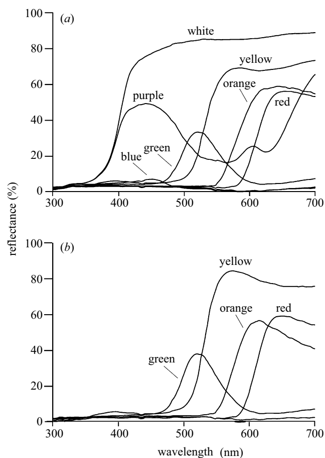
Figure 1. Reflectance spectra of the coloured discs used in (a) the first field study and in the laboratory experiment (clear plastic) and (b) the second field study (metal coins).
