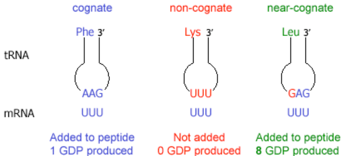
Figure Z.13 Results of the experiment by Thompson and Stone to verify Hopfield's mechanism.
