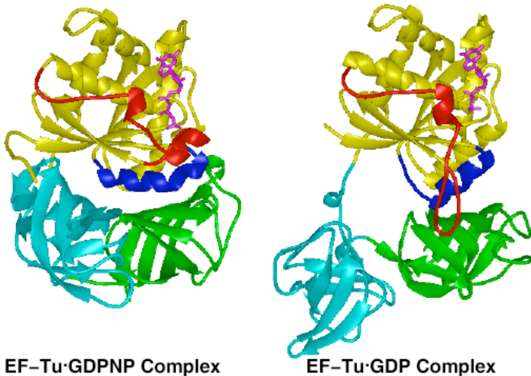
Figure Z.12 Conformational changes associated with GTP hydrolysis. Domain I is in yellow, domain II in green and domain III in turquoise. The flexible loop and mobile helix are red and blue, respectively.
