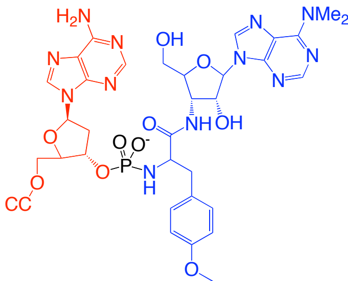
Figure Z.14 Structure of the CCdA-p-Puro inhibitor of the transpeptidation reaction.
