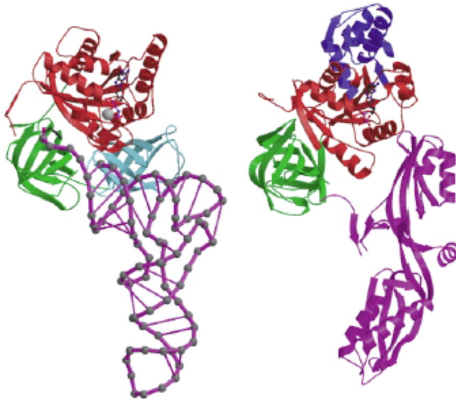
Figure Z.16 Comparison of the structure of EF-Tu•GTP•aa-tRNA on the left and EF-G on the right. The C-terminal domains of EF-G adopt a fold that is strikingly similar to the tRNA structure.
