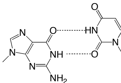
Figure Z.6 The wobble base pair between guanine and uracil.
